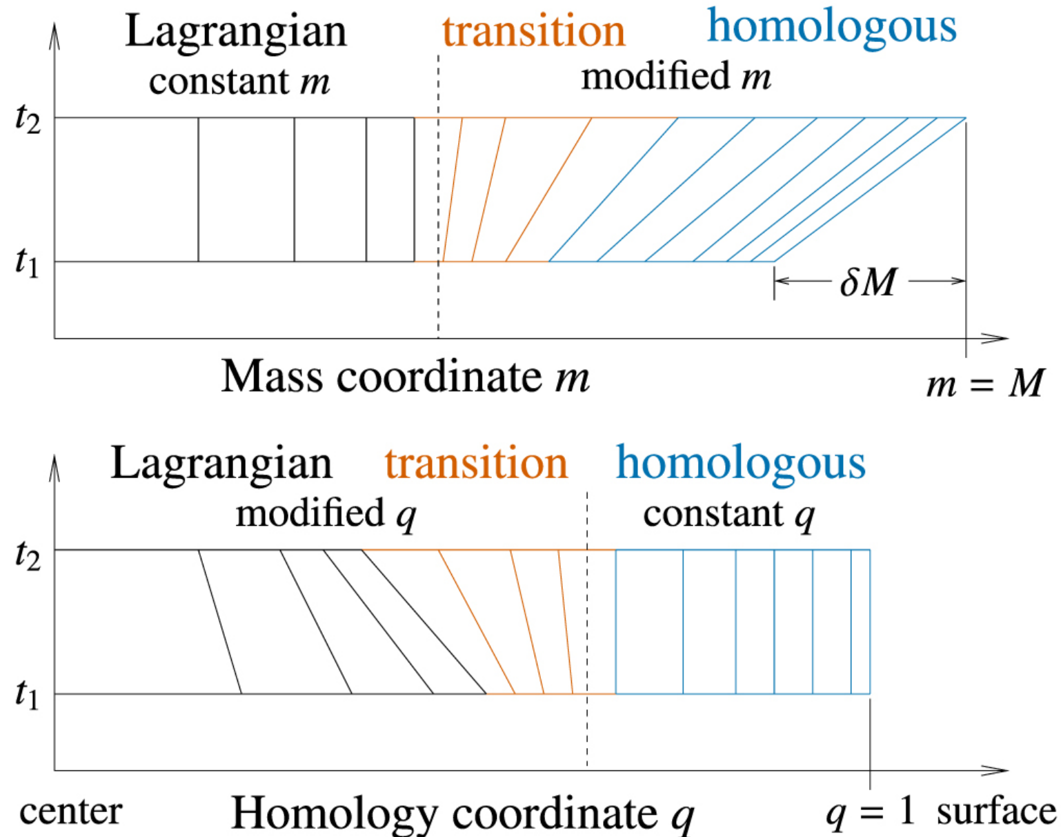
Figure 32. from MODULES FOR EXPERIMENTS IN STELLAR ASTROPHYSICS (MESA): BINARIES, PULSATIONS, AND EXPLOSIONS null 2015 APJS 220 15 doi:10.1088/0067-0049/220/1/15 https://dx.doi.org/10.1088/0067-0049/220/1/15 © 2015. The American Astronomical Society. All rights reserved.
