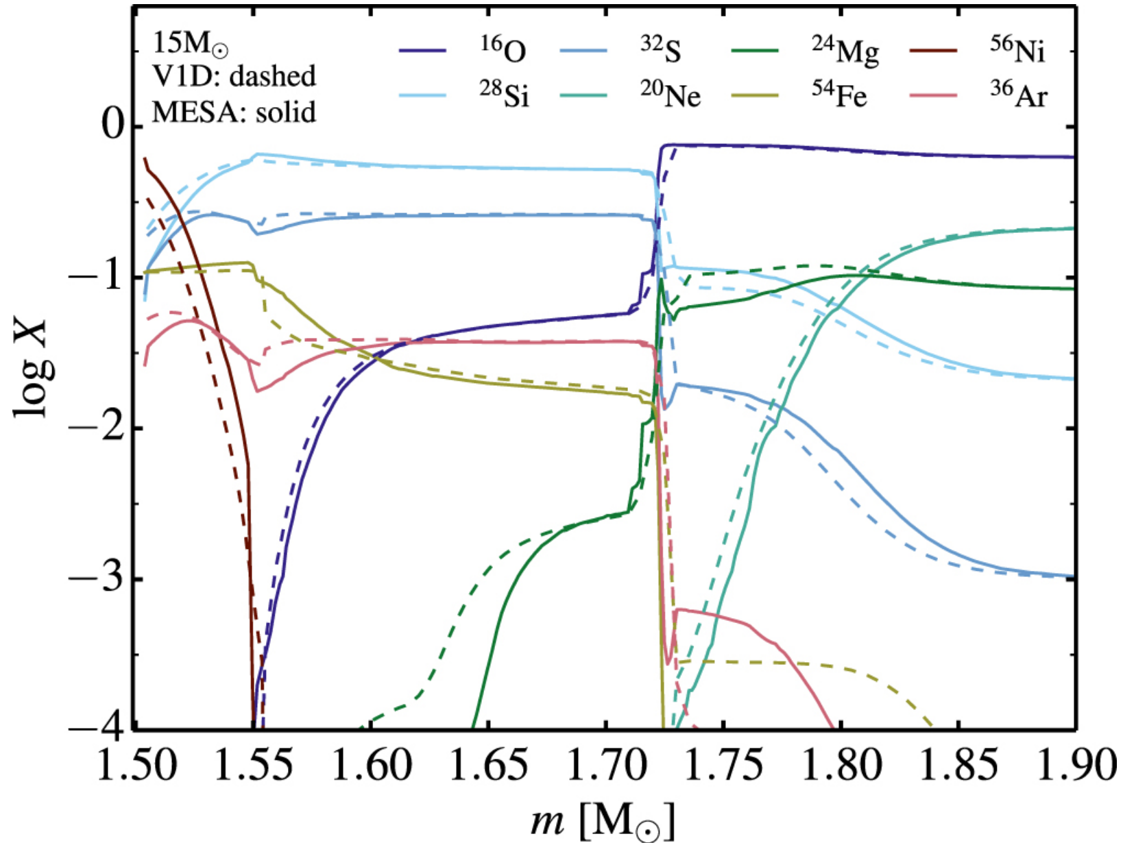
Figure 31. from MODULES FOR EXPERIMENTS IN STELLAR ASTROPHYSICS (MESA): BINARIES, PULSATIONS, AND EXPLOSIONS null 2015 APJS 220 15 doi:10.1088/0067-0049/220/1/15 https://dx.doi.org/10.1088/0067-0049/220/1/15 © 2015. The American Astronomical Society. All rights reserved.
