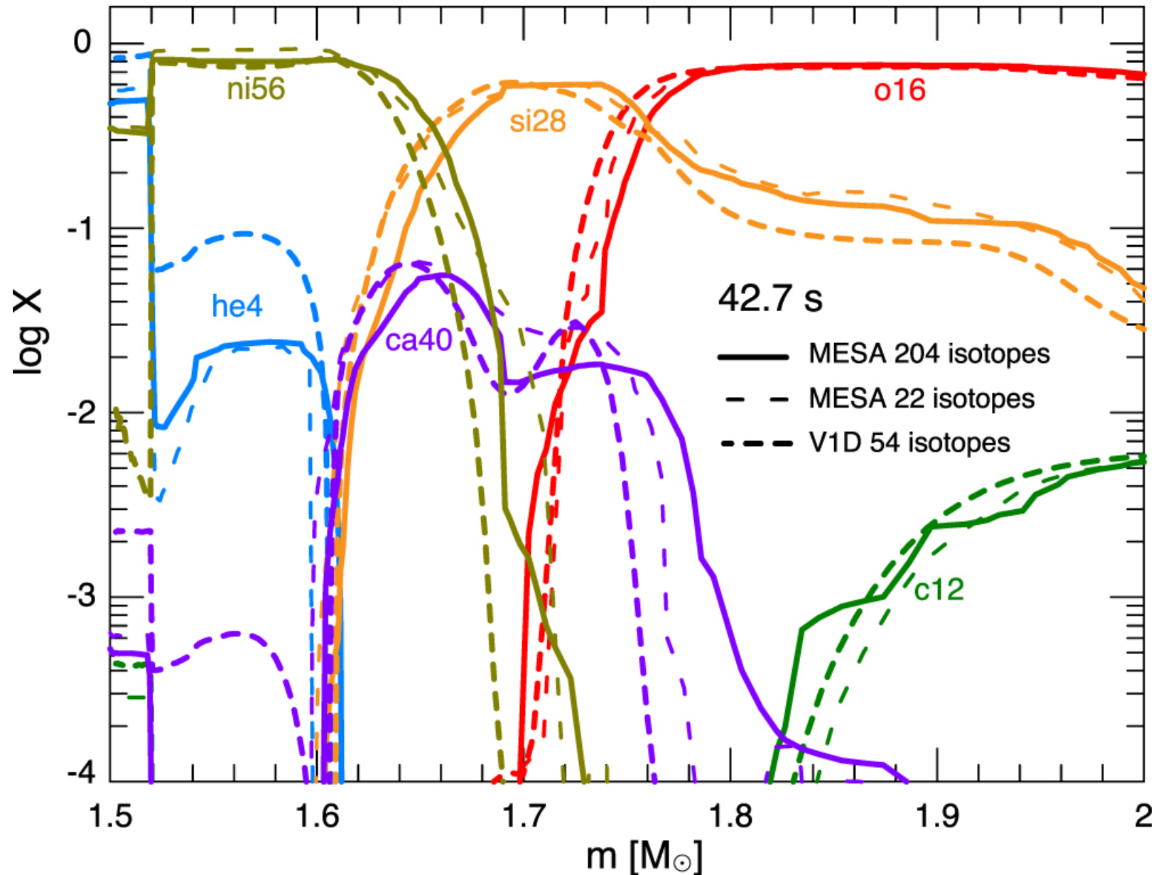
Figure 30. from MODULES FOR EXPERIMENTS IN STELLAR ASTROPHYSICS (MESA): BINARIES, PULSATIONS, AND EXPLOSIONS null 2015 APJS 220 15 doi:10.1088/0067-0049/220/1/15 https://dx.doi.org/10.1088/0067-0049/220/1/15 © 2015. The American Astronomical Society. All rights reserved.
