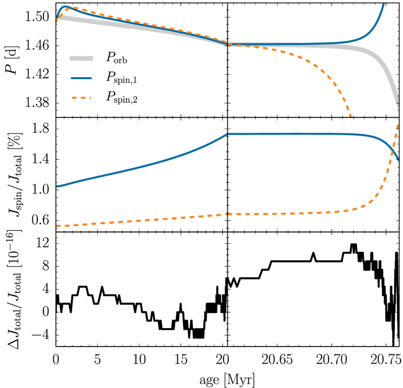
Figure 3. from MODULES FOR EXPERIMENTS IN STELLAR ASTROPHYSICS (MESA): BINARIES, PULSATIONS, AND EXPLOSIONS null 2015 APJS 220 15 doi:10.1088/0067-0049/220/1/15 https://dx.doi.org/10.1088/0067-0049/220/1/15 © 2015. The American Astronomical Society. All rights reserved.
