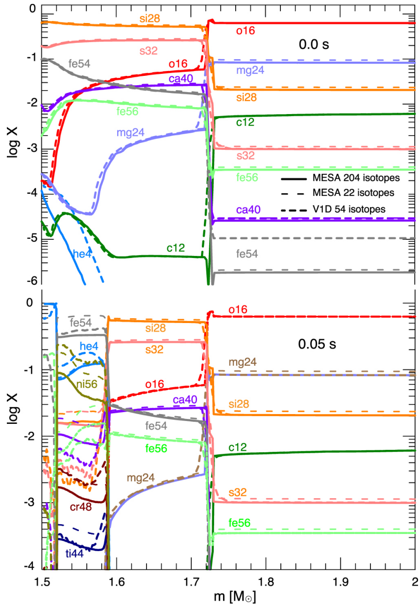
Figure 29. from MODULES FOR EXPERIMENTS IN STELLAR ASTROPHYSICS (MESA): BINARIES, PULSATIONS, AND EXPLOSIONS null 2015 APJS 220 15 doi:10.1088/0067-0049/220/1/15 https://dx.doi.org/10.1088/0067-0049/220/1/15 © 2015. The American Astronomical Society. All rights reserved.
