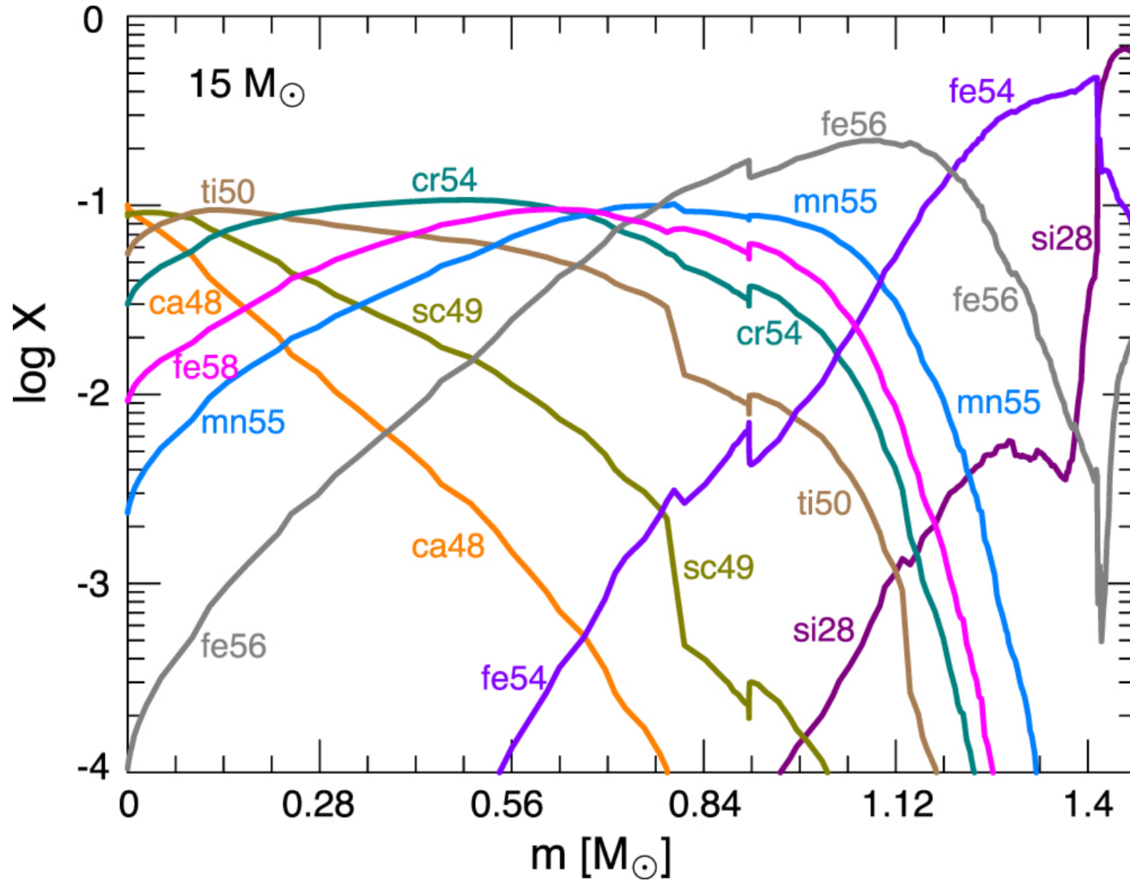
Figure 27. from MODULES FOR EXPERIMENTS IN STELLAR ASTROPHYSICS (MESA): BINARIES, PULSATIONS, AND EXPLOSIONS null 2015 APJS 220 15 doi:10.1088/0067-0049/220/1/15 https://dx.doi.org/10.1088/0067-0049/220/1/15 © 2015. The American Astronomical Society. All rights reserved.
