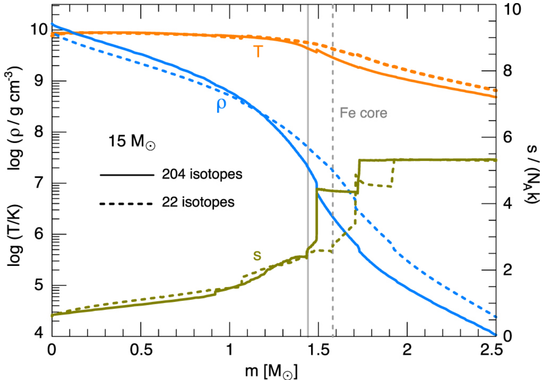
Figure 26. from MODULES FOR EXPERIMENTS IN STELLAR ASTROPHYSICS (MESA): BINARIES, PULSATIONS, AND EXPLOSIONS null 2015 APJS 220 15 doi:10.1088/0067-0049/220/1/15 https://dx.doi.org/10.1088/0067-0049/220/1/15 © 2015. The American Astronomical Society. All rights reserved.
