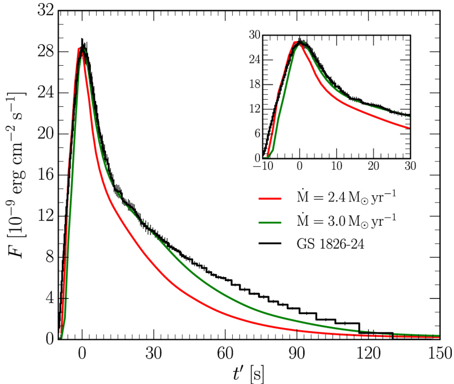
Figure 23. from MODULES FOR EXPERIMENTS IN STELLAR ASTROPHYSICS (MESA): BINARIES, PULSATIONS, AND EXPLOSIONS null 2015 APJS 220 15 doi:10.1088/0067-0049/220/1/15 https://dx.doi.org/10.1088/0067-0049/220/1/15 © 2015. The American Astronomical Society. All rights reserved.
