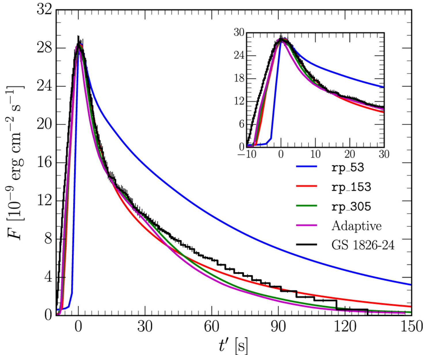
Figure 22. from MODULES FOR EXPERIMENTS IN STELLAR ASTROPHYSICS (MESA): BINARIES, PULSATIONS, AND EXPLOSIONS null 2015 APJS 220 15 doi:10.1088/0067-0049/220/1/15 https://dx.doi.org/10.1088/0067-0049/220/1/15 © 2015. The American Astronomical Society. All rights reserved.
