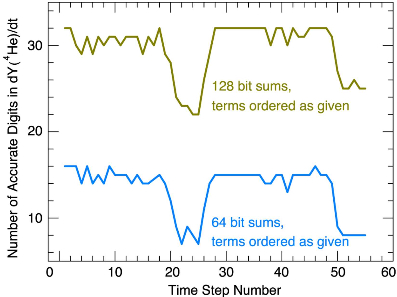
Figure 20. from MODULES FOR EXPERIMENTS IN STELLAR ASTROPHYSICS (MESA): BINARIES, PULSATIONS, AND EXPLOSIONS null 2015 APJS 220 15 doi:10.1088/0067-0049/220/1/15 https://dx.doi.org/10.1088/0067-0049/220/1/15 © 2015. The American Astronomical Society. All rights reserved.
