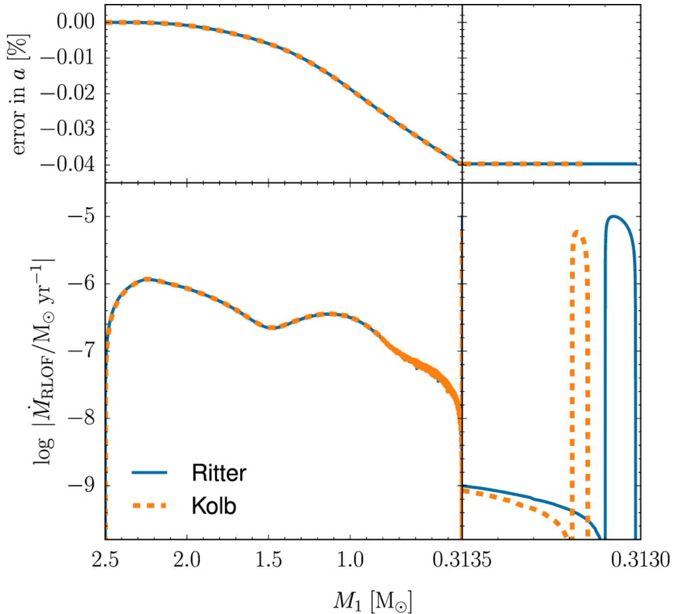
Figure 2. from MODULES FOR EXPERIMENTS IN STELLAR ASTROPHYSICS (MESA): BINARIES, PULSATIONS, AND EXPLOSIONS null 2015 APJS 220 15 doi:10.1088/0067-0049/220/1/15 https://dx.doi.org/10.1088/0067-0049/220/1/15 © 2015. The American Astronomical Society. All rights reserved.
