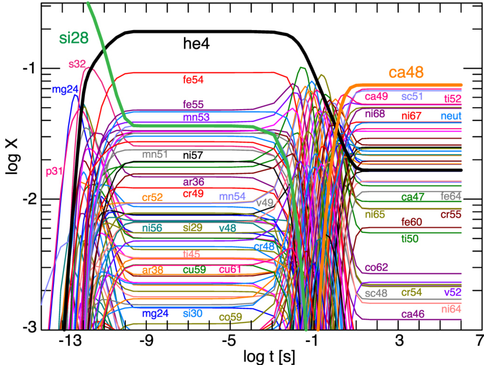
Figure 19. from MODULES FOR EXPERIMENTS IN STELLAR ASTROPHYSICS (MESA): BINARIES, PULSATIONS, AND EXPLOSIONS null 2015 APJS 220 15 doi:10.1088/0067-0049/220/1/15 https://dx.doi.org/10.1088/0067-0049/220/1/15 © 2015. The American Astronomical Society. All rights reserved.
