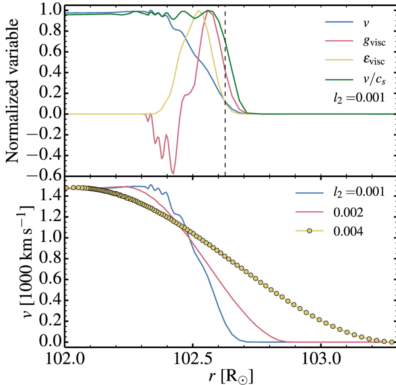
Figure 18. from MODULES FOR EXPERIMENTS IN STELLAR ASTROPHYSICS (MESA): BINARIES, PULSATIONS, AND EXPLOSIONS null 2015 APJS 220 15 doi:10.1088/0067-0049/220/1/15 https://dx.doi.org/10.1088/0067-0049/220/1/15 © 2015. The American Astronomical Society. All rights reserved.
