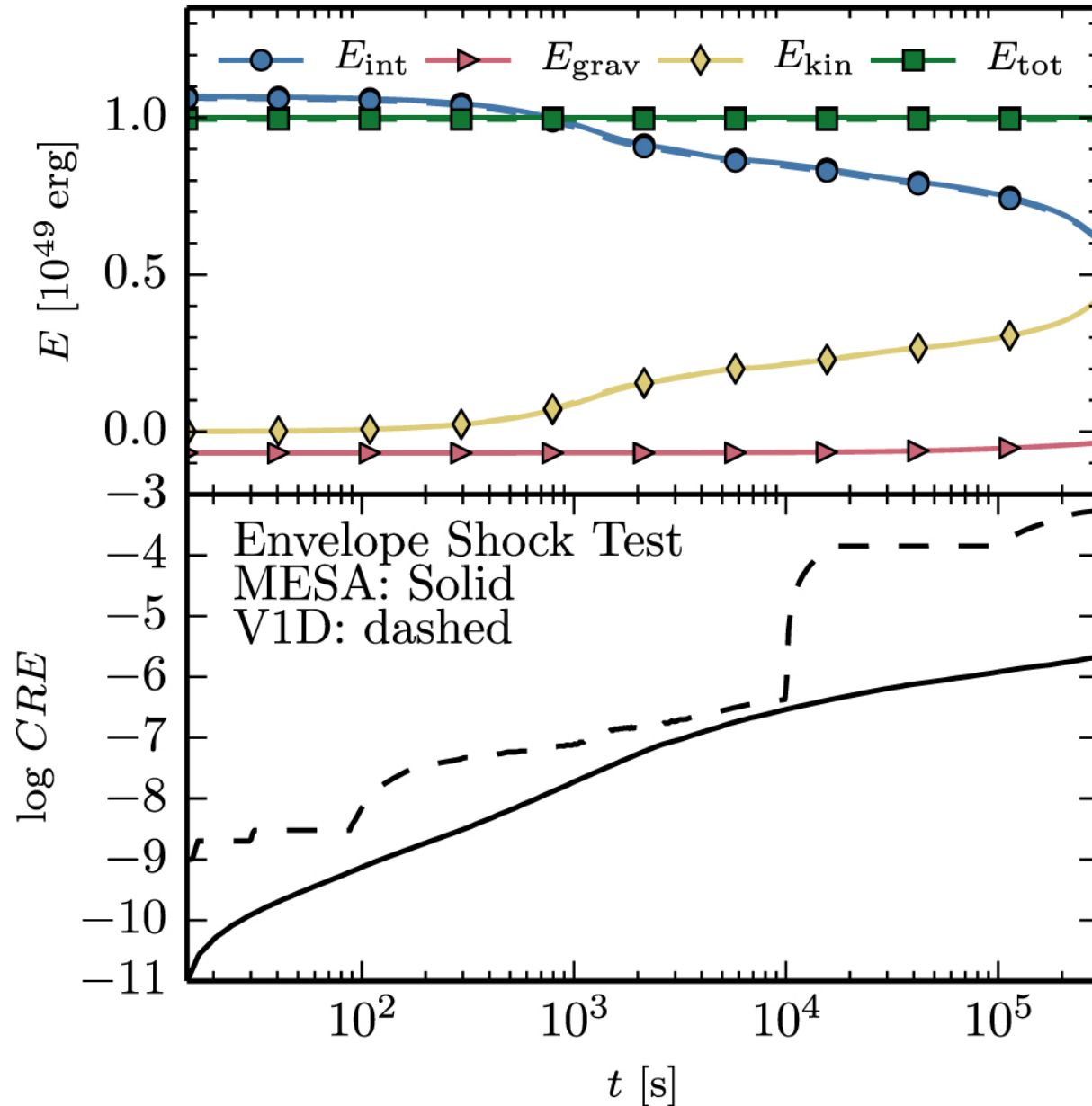
Figure 17. from MODULES FOR EXPERIMENTS IN STELLAR ASTROPHYSICS (MESA): BINARIES, PULSATIONS, AND EXPLOSIONS null 2015 APJS 220 15 doi:10.1088/0067-0049/220/1/15 https://dx.doi.org/10.1088/0067-0049/220/1/15 © 2015. The American Astronomical Society. All rights reserved.
