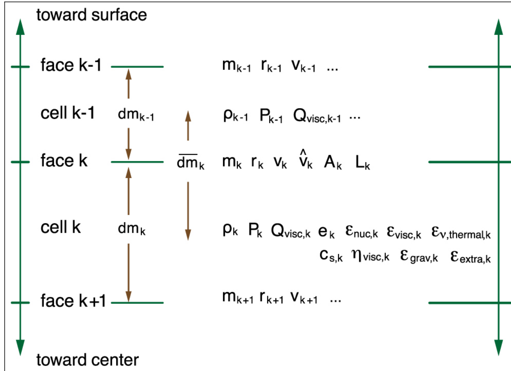
Figure 15. from MODULES FOR EXPERIMENTS IN STELLAR ASTROPHYSICS (MESA): BINARIES, PULSATIONS, AND EXPLOSIONS null 2015 APJS 220 15 doi:10.1088/0067-0049/220/1/15 https://dx.doi.org/10.1088/0067-0049/220/1/15 © 2015. The American Astronomical Society. All rights reserved.
