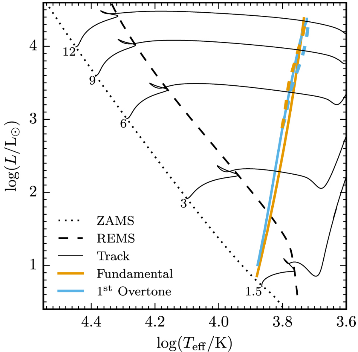
Figure 14. from MODULES FOR EXPERIMENTS IN STELLAR ASTROPHYSICS (MESA): BINARIES, PULSATIONS, AND EXPLOSIONS null 2015 APJS 220 15 doi:10.1088/0067-0049/220/1/15 https://dx.doi.org/10.1088/0067-0049/220/1/15 © 2015. The American Astronomical Society. All rights reserved.
