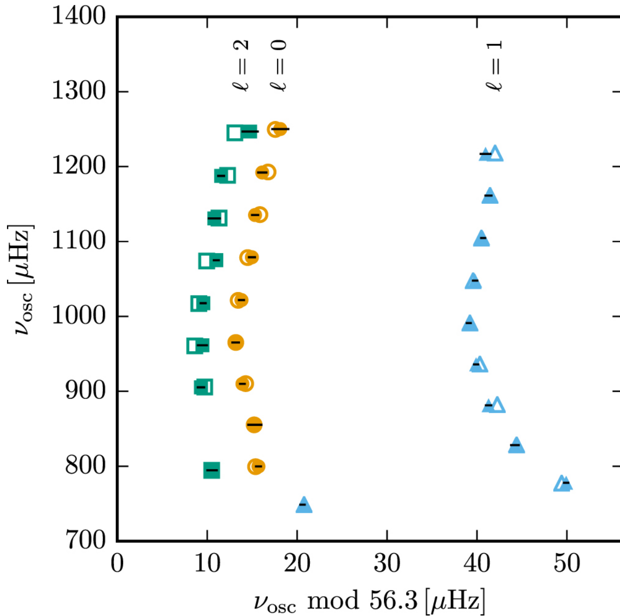
Figure 12. from MODULES FOR EXPERIMENTS IN STELLAR ASTROPHYSICS (MESA): BINARIES, PULSATIONS, AND EXPLOSIONS null 2015 APJS 220 15 doi:10.1088/0067-0049/220/1/15 https://dx.doi.org/10.1088/0067-0049/220/1/15 © 2015. The American Astronomical Society. All rights reserved.
