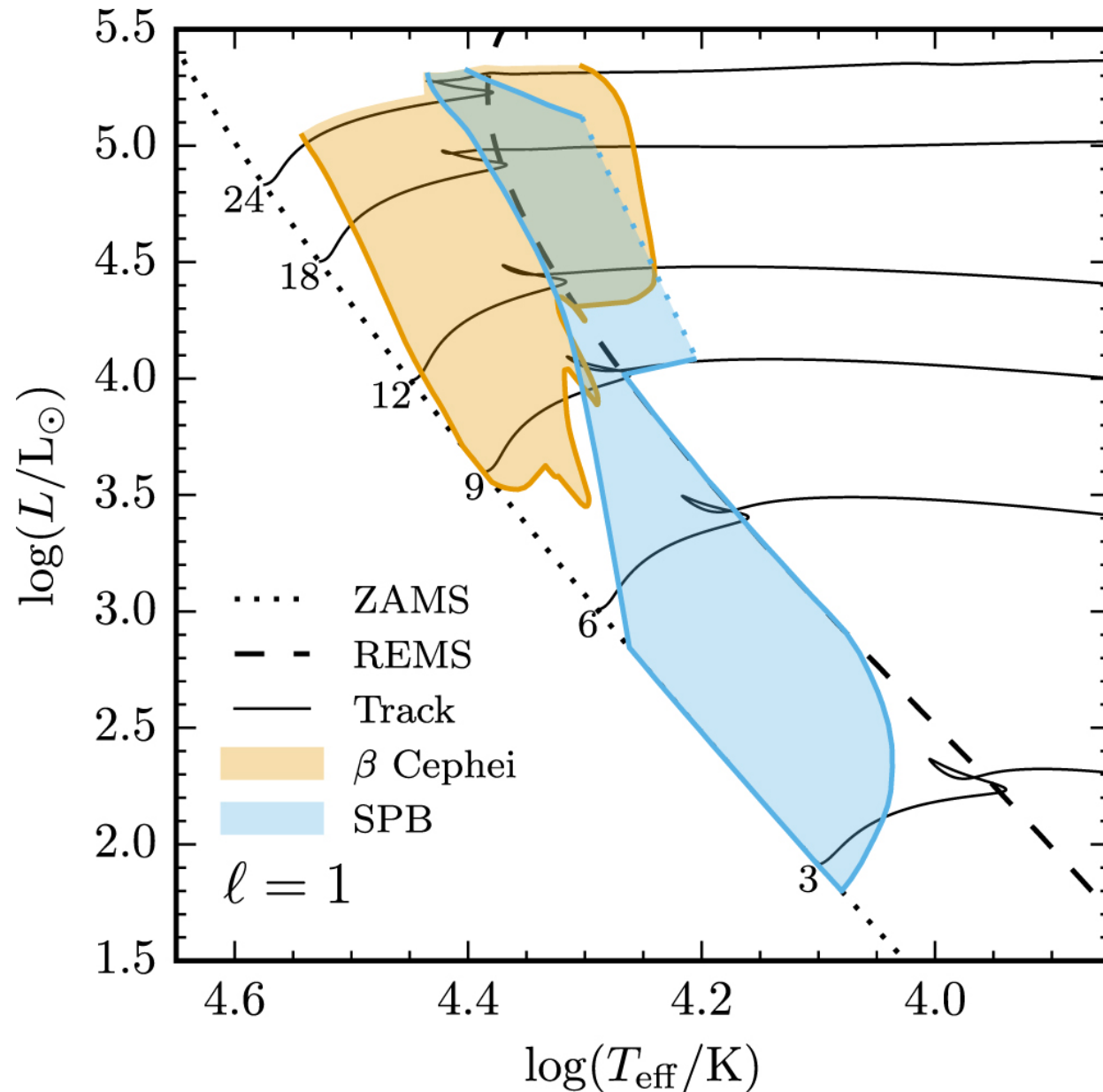
Figure 11. from MODULES FOR EXPERIMENTS IN STELLAR ASTROPHYSICS (MESA): BINARIES, PULSATIONS, AND EXPLOSIONS null 2015 APJS 220 15 doi:10.1088/0067-0049/220/1/15 https://dx.doi.org/10.1088/0067-0049/220/1/15 © 2015. The American Astronomical Society. All rights reserved.
