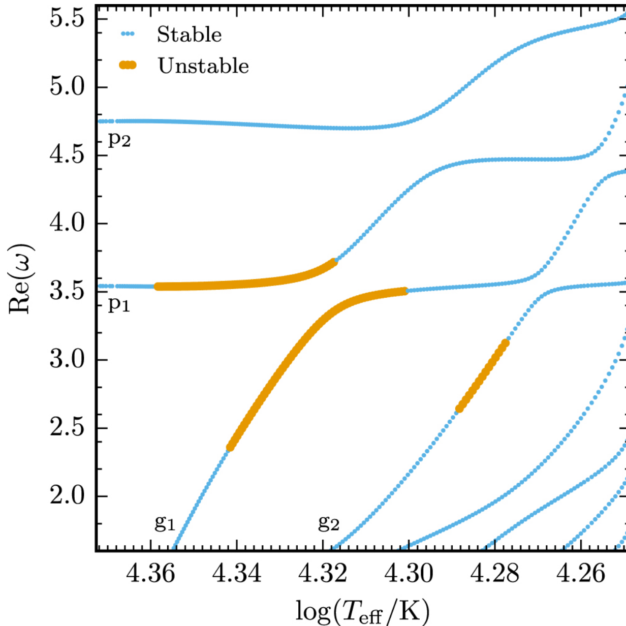
Figure 10. from MODULES FOR EXPERIMENTS IN STELLAR ASTROPHYSICS (MESA): BINARIES, PULSATIONS, AND EXPLOSIONS null 2015 APJS 220 15 doi:10.1088/0067-0049/220/1/15 https://dx.doi.org/10.1088/0067-0049/220/1/15 © 2015. The American Astronomical Society. All rights reserved.
