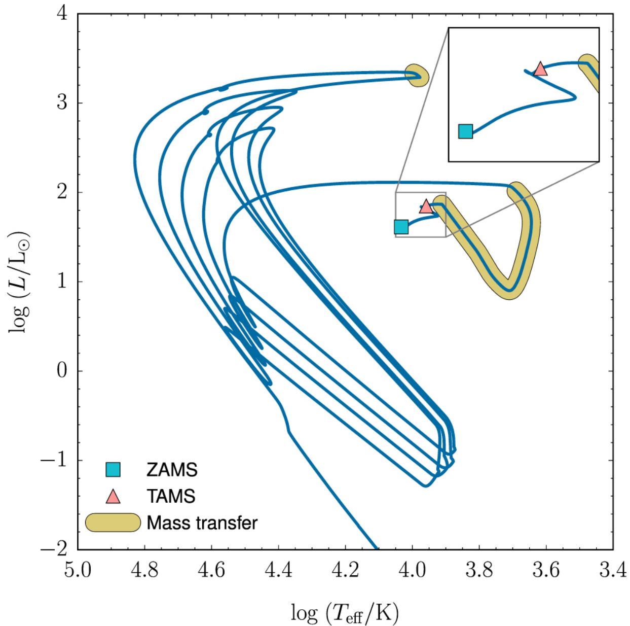
Figure 1. from MODULES FOR EXPERIMENTS IN STELLAR ASTROPHYSICS (MESA): BINARIES, PULSATIONS, AND EXPLOSIONS null 2015 APJS 220 15 doi:10.1088/0067-0049/220/1/15 https://dx.doi.org/10.1088/0067-0049/220/1/15 © 2015. The American Astronomical Society. All rights reserved.
