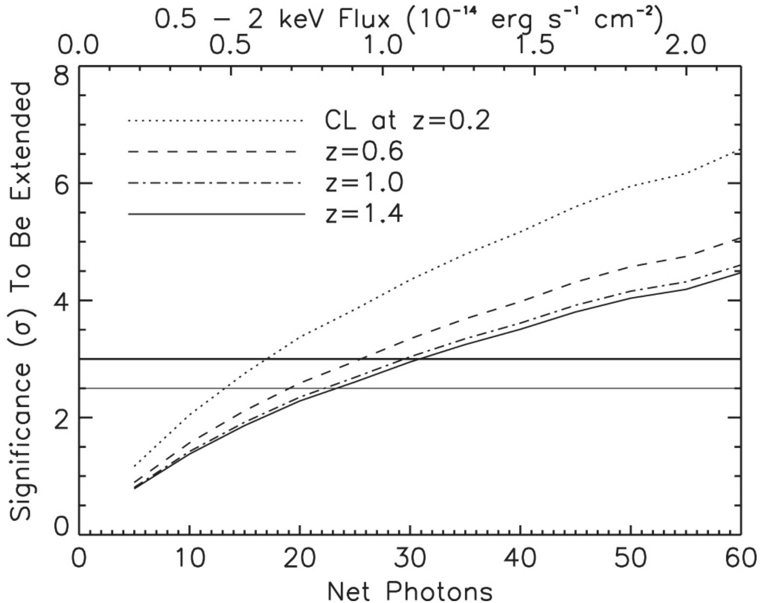
Figure 6. from THE SWIFT AGN AND CLUSTER SURVEY. I. NUMBER COUNTS OF AGNs AND GALAXY CLUSTERS null 2015 APJS 218 8 doi:10.1088/0067-0049/218/1/8 https://dx.doi.org/10.1088/0067-0049/218/1/8 © 2015. The American Astronomical Society. All rights reserved.
