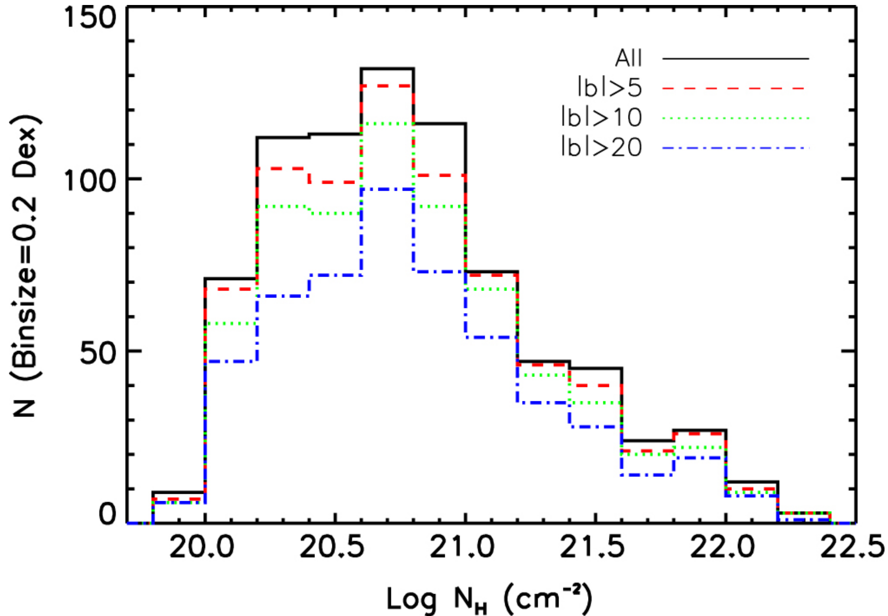
Figure 4. from THE SWIFT AGN AND CLUSTER SURVEY. I. NUMBER COUNTS OF AGNs AND GALAXY CLUSTERS null 2015 APJS 218 8 doi:10.1088/0067-0049/218/1/8 https://dx.doi.org/10.1088/0067-0049/218/1/8 © 2015. The American Astronomical Society. All rights reserved.
