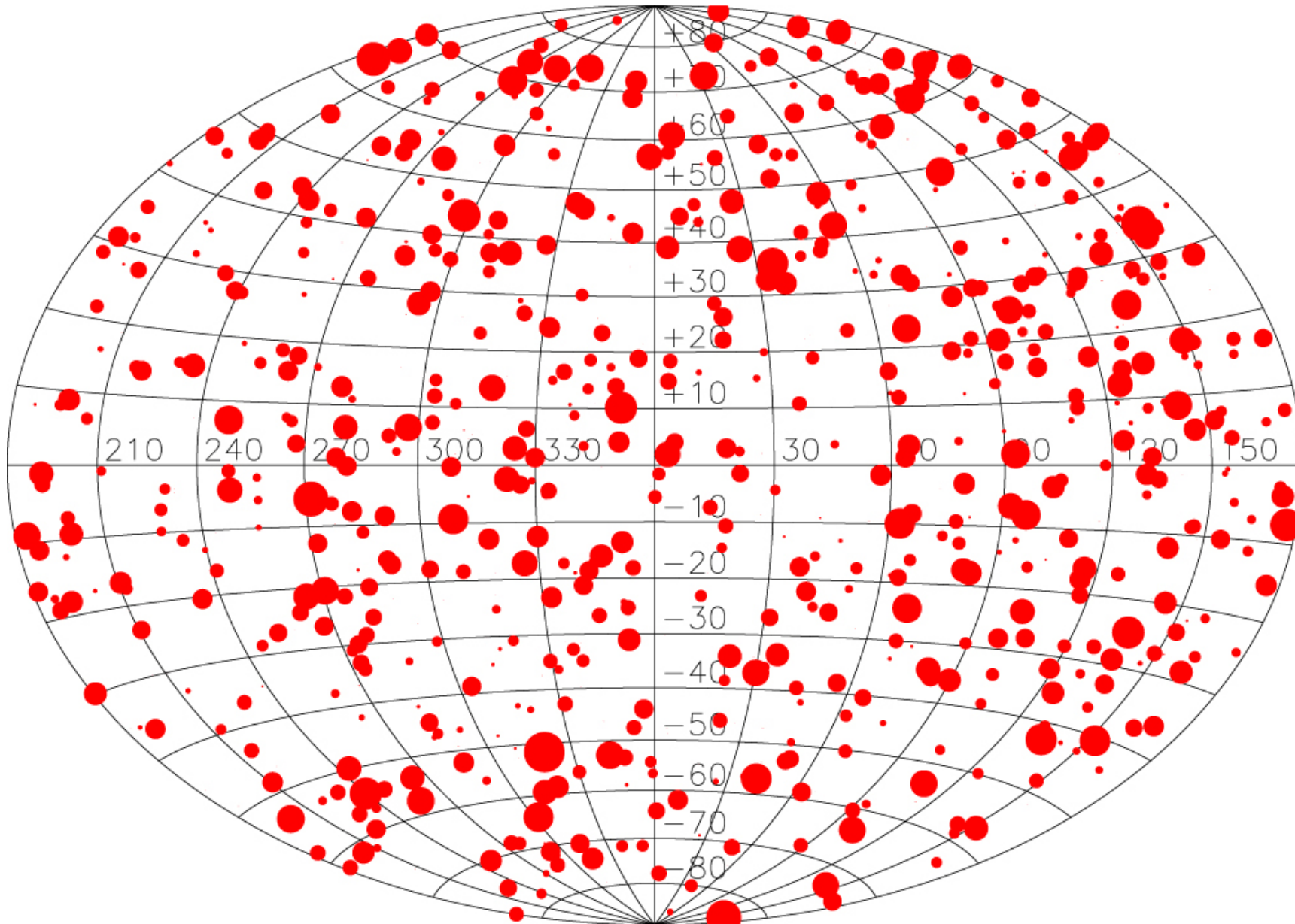
Figure 2. from THE SWIFT AGN AND CLUSTER SURVEY. I. NUMBER COUNTS OF AGNs AND GALAXY CLUSTERS null 2015 APJS 218 8 doi:10.1088/0067-0049/218/1/8 https://dx.doi.org/10.1088/0067-0049/218/1/8 © 2015. The American Astronomical Society. All rights reserved.
