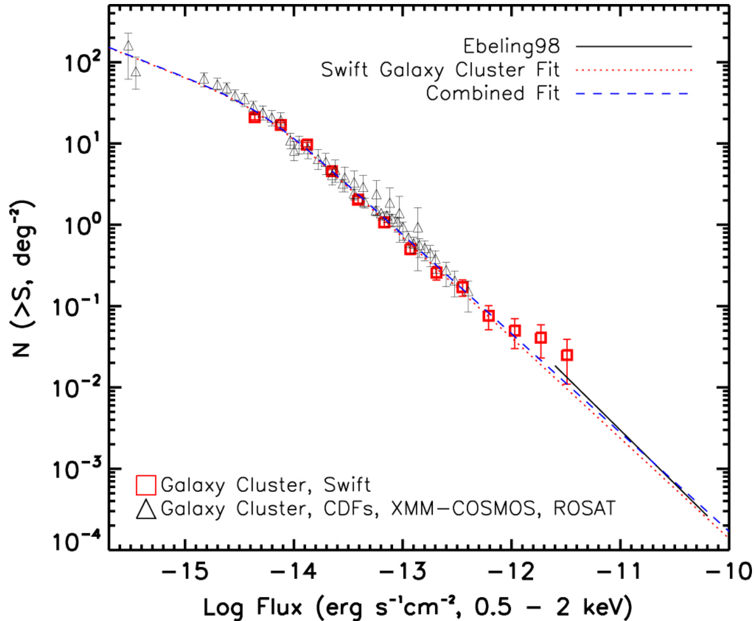
Figure 18. from THE SWIFT AGN AND CLUSTER SURVEY. I. NUMBER COUNTS OF AGNs AND GALAXY CLUSTERS null 2015 APJS 218 8 doi:10.1088/0067-0049/218/1/8 https://dx.doi.org/10.1088/0067-0049/218/1/8 © 2015. The American Astronomical Society. All rights reserved.
