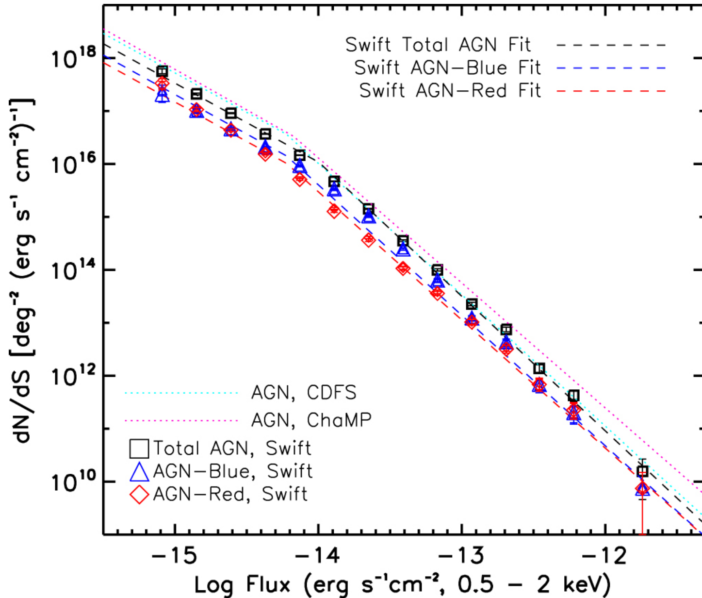
Figure 16. from THE SWIFT AGN AND CLUSTER SURVEY. I. NUMBER COUNTS OF AGNs AND GALAXY CLUSTERS null 2015 APJS 218 8 doi:10.1088/0067-0049/218/1/8 https://dx.doi.org/10.1088/0067-0049/218/1/8 © 2015. The American Astronomical Society. All rights reserved.
