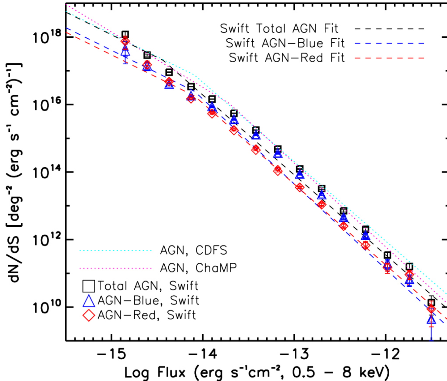
Figure 15. from THE SWIFT AGN AND CLUSTER SURVEY. I. NUMBER COUNTS OF AGNs AND GALAXY CLUSTERS null 2015 APJS 218 8 doi:10.1088/0067-0049/218/1/8 https://dx.doi.org/10.1088/0067-0049/218/1/8 © 2015. The American Astronomical Society. All rights reserved.
