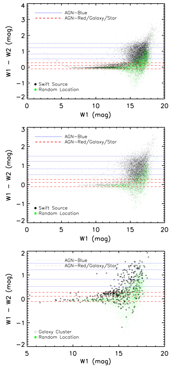
Figure 10. from THE SWIFT AGN AND CLUSTER SURVEY. I. NUMBER COUNTS OF AGNs AND GALAXY CLUSTERS null 2015 APJS 218 8 doi:10.1088/0067-0049/218/1/8 https://dx.doi.org/10.1088/0067-0049/218/1/8 © 2015. The American Astronomical Society. All rights reserved.
