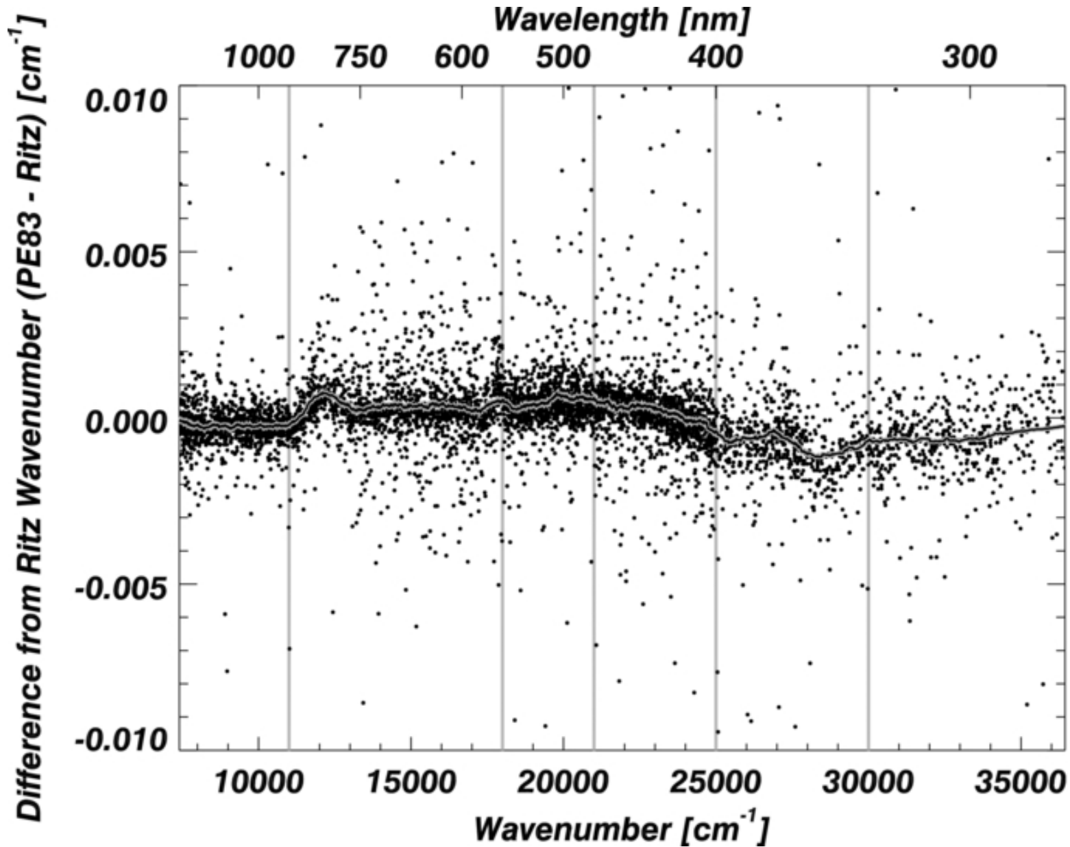
Figure 8. from The Spectrum of Thorium from 250 nm to 5500 nm: Ritz Wavelengths and Optimized Energy Levels Redman, Nave, & Sansonetti 2014 ApJS 211 4 doi:10.1088/0067-0049/211/1/4 https://dx.doi.org/10.1088/0067-0049/211/1/4 © 2014. The American Astronomical Society. All rights reserved.
