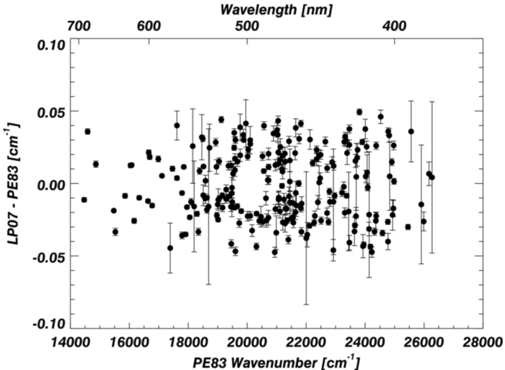
Figure 7. from The Spectrum of Thorium from 250 nm to 5500 nm: Ritz Wavelengths and Optimized Energy Levels Redman, Nave, & Sansonetti 2014 ApJS 211 4 doi:10.1088/0067-0049/211/1/4 https://dx.doi.org/10.1088/0067-0049/211/1/4 © 2014. The American Astronomical Society. All rights reserved.
