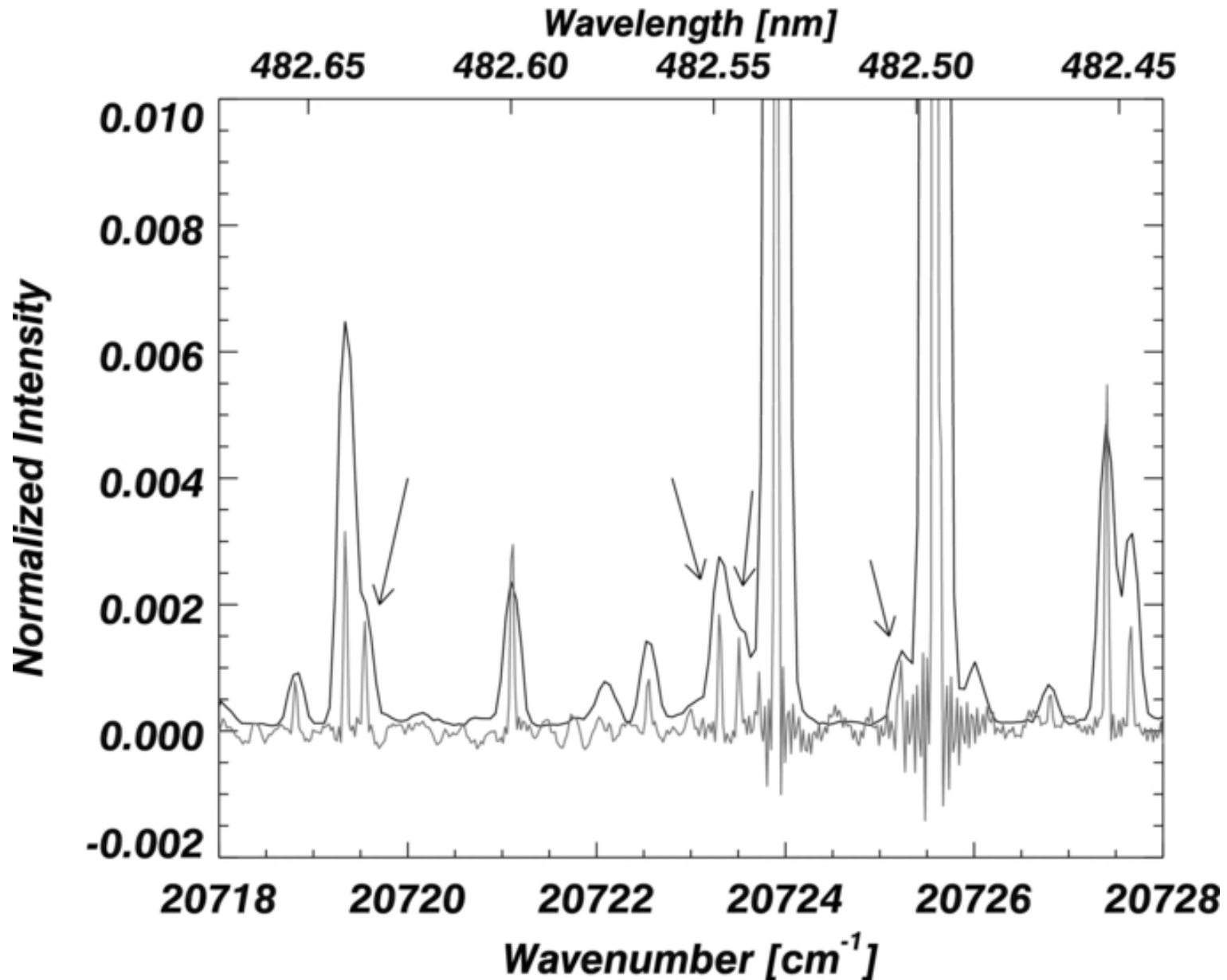
Figure 6. from The Spectrum of Thorium from 250 nm to 5500 nm: Ritz Wavelengths and Optimized Energy Levels Redman, Nave, & Sansonetti 2014 ApJS 211 4 doi:10.1088/0067-0049/211/1/4 https://dx.doi.org/10.1088/0067-0049/211/1/4 © 2014. The American Astronomical Society. All rights reserved.
