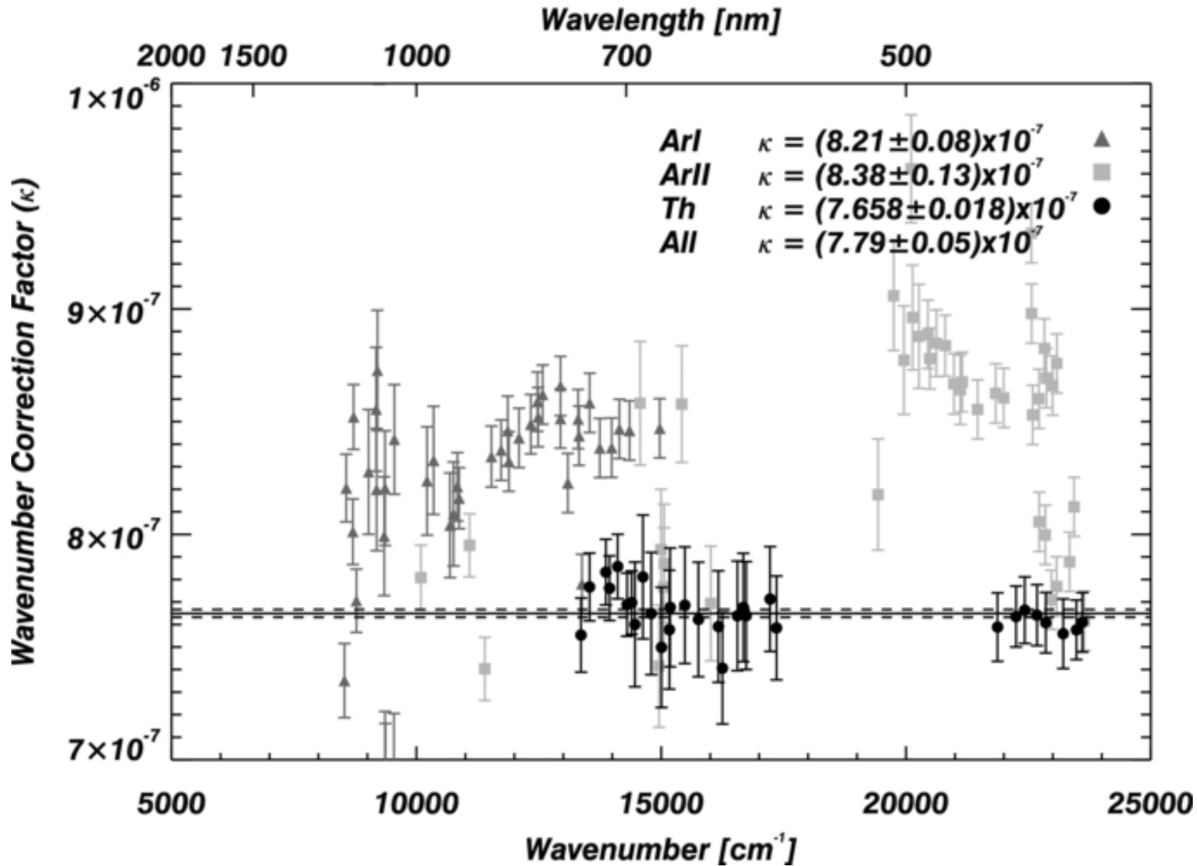
Figure 2. from The Spectrum of Thorium from 250 nm to 5500 nm: Ritz Wavelengths and Optimized Energy Levels Redman, Nave, & Sansonetti 2014 ApJS 211 4 doi:10.1088/0067-0049/211/1/4 https://dx.doi.org/10.1088/0067-0049/211/1/4 © 2014. The American Astronomical Society. All rights reserved.
