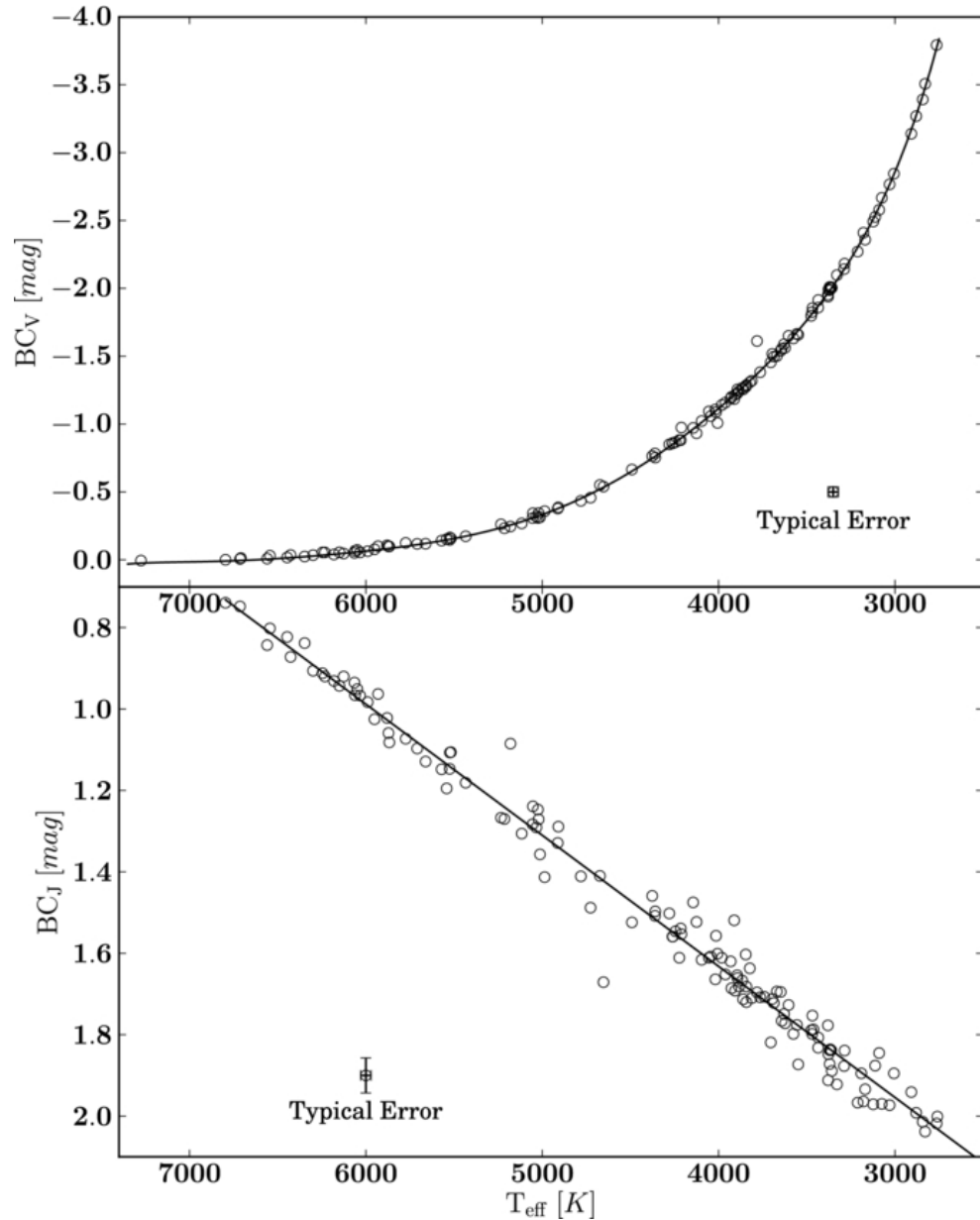
Figure 8. from Intrinsic Colors, Temperatures, and Bolometric Corrections of Pre-main-sequence Stars Pecaut & Mamajek 2013 ApJS 208 9 doi:10.1088/0067-0049/208/1/9 https://dx.doi.org/10.1088/0067-0049/208/1/9 © 2013. The American Astronomical Society. All rights reserved.
