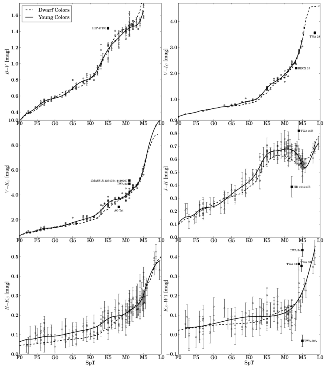
Figure 4. from Intrinsic Colors, Temperatures, and Bolometric Corrections of Pre-main-sequence Stars Pecaut & Mamajek 2013 ApJS 208 9 doi:10.1088/0067-0049/208/1/9 https://dx.doi.org/10.1088/0067-0049/208/1/9 © 2013. The American Astronomical Society. All rights reserved.
