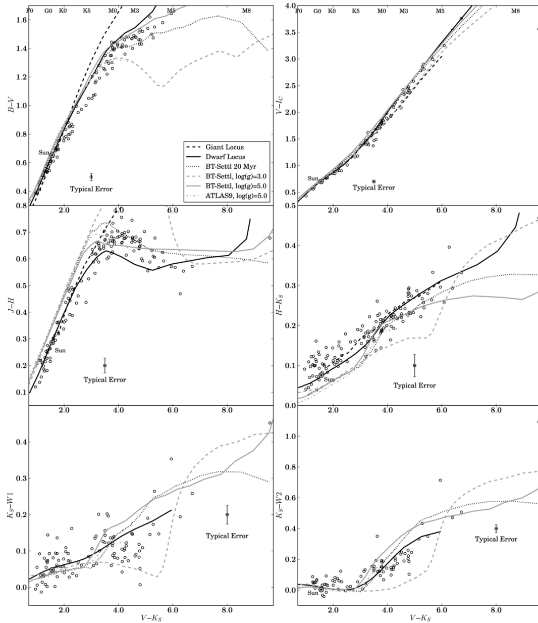
Figure 2. from Intrinsic Colors, Temperatures, and Bolometric Corrections of Pre-main-sequence Stars Pecaut & Mamajek 2013 ApJS 208 9 doi:10.1088/0067-0049/208/1/9 https://dx.doi.org/10.1088/0067-0049/208/1/9 © 2013. The American Astronomical Society. All rights reserved.
