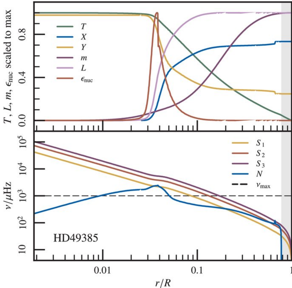
Figure 9. from Modules for Experiments in Stellar Astrophysics (MESA): Planets, Oscillations, Rotation, and Massive Stars Paxton et al. 2013 ApJS 208 4 doi:10.1088/0067-0049/208/1/4 https://dx.doi.org/10.1088/0067-0049/208/1/4 © 2013. The American Astronomical Society. All rights reserved.
