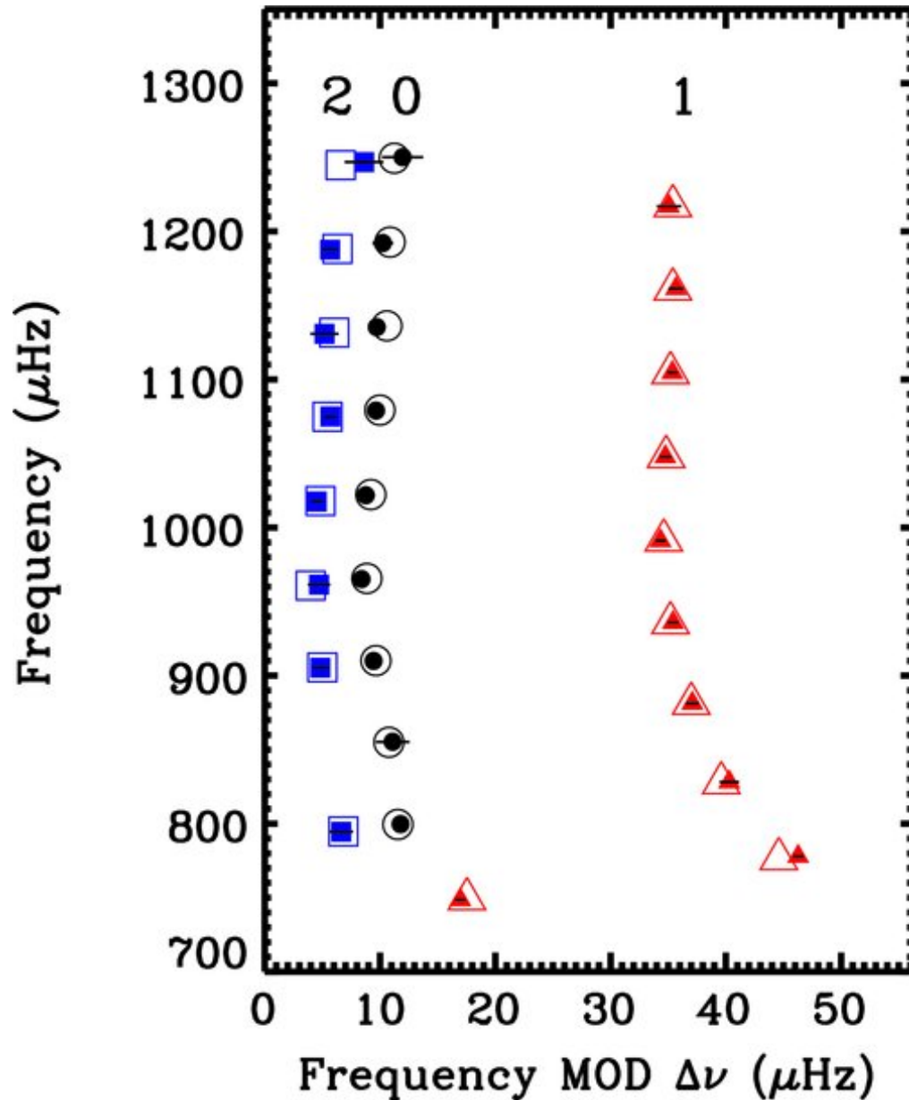
Figure 8. from Modules for Experiments in Stellar Astrophysics (MESA): Planets, Oscillations, Rotation, and Massive Stars Paxton et al. 2013 ApJS 208 4 doi:10.1088/0067-0049/208/1/4 https://dx.doi.org/10.1088/0067-0049/208/1/4 © 2013. The American Astronomical Society. All rights reserved.
