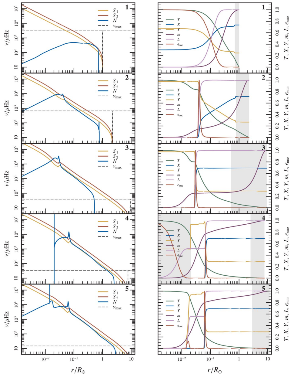
Figure 6. from Modules for Experiments in Stellar Astrophysics (MESA): Planets, Oscillations, Rotation, and Massive Stars Paxton et al. 2013 ApJS 208 4 doi:10.1088/0067-0049/208/1/4 https://dx.doi.org/10.1088/0067-0049/208/1/4 © 2013. The American Astronomical Society. All rights reserved.
