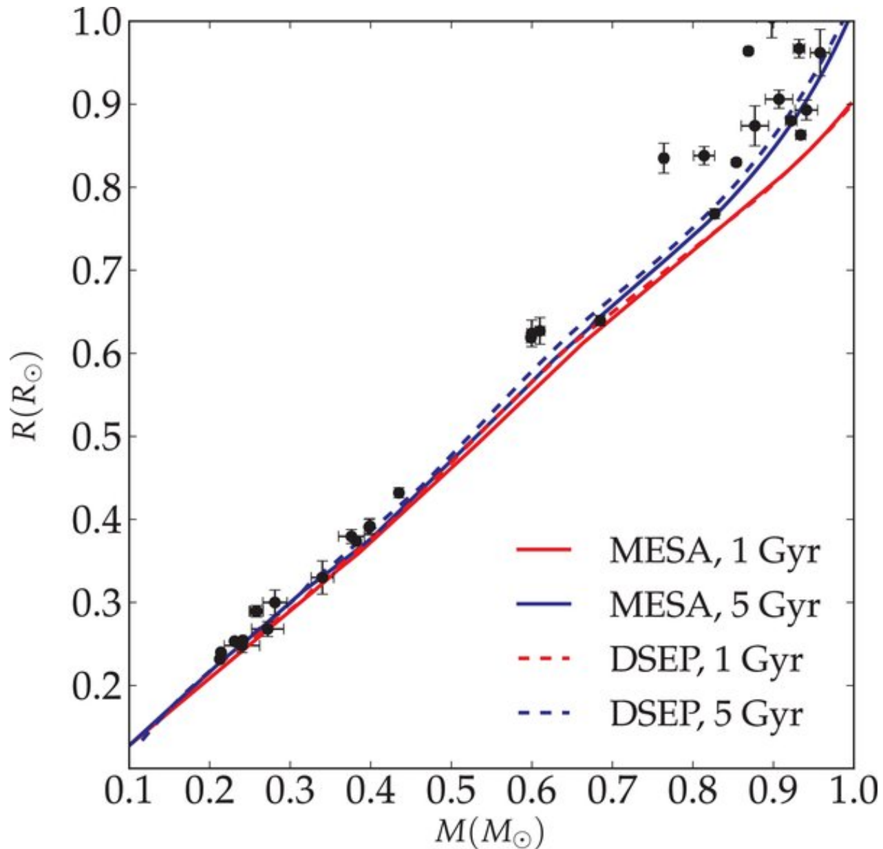
Figure 4. from Modules for Experiments in Stellar Astrophysics (MESA): Planets, Oscillations, Rotation, and Massive Stars Paxton et al. 2013 ApJS 208 4 doi:10.1088/0067-0049/208/1/4 https://dx.doi.org/10.1088/0067-0049/208/1/4 © 2013. The American Astronomical Society. All rights reserved.
