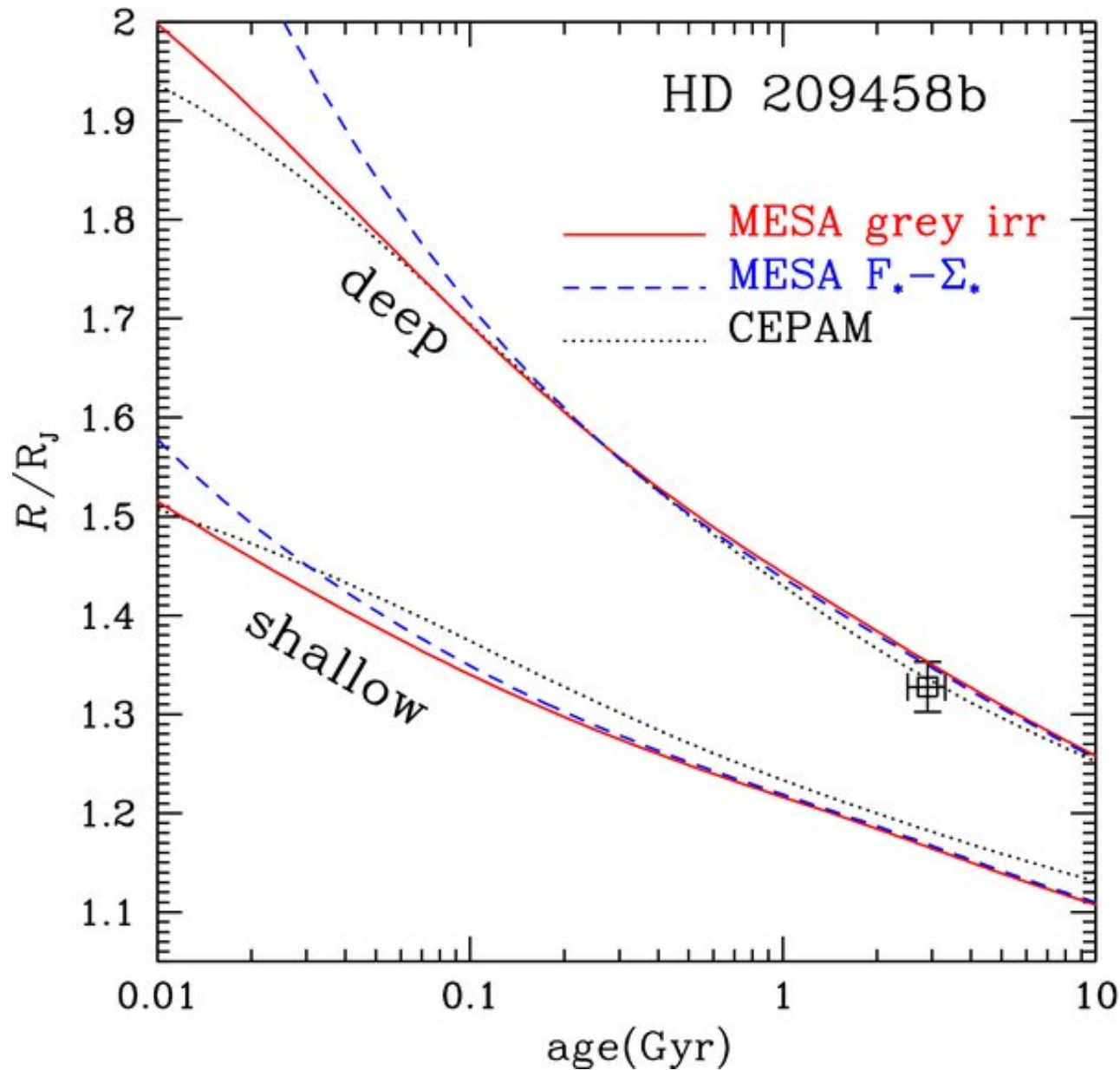
Figure 3. from Modules for Experiments in Stellar Astrophysics (MESA): Planets, Oscillations, Rotation, and Massive Stars Paxton et al. 2013 ApJS 208 4 doi:10.1088/0067-0049/208/1/4 https://dx.doi.org/10.1088/0067-0049/208/1/4 © 2013. The American Astronomical Society. All rights reserved.
