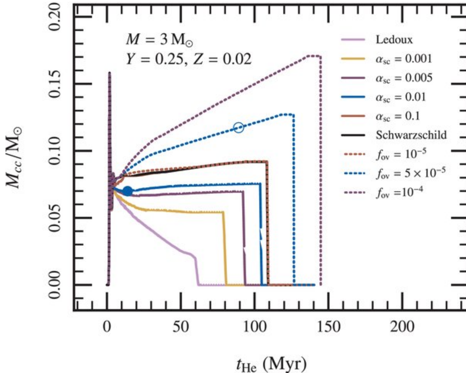
Figure 15. from Modules for Experiments in Stellar Astrophysics (MESA): Planets, Oscillations, Rotation, and Massive Stars Paxton et al. 2013 ApJS 208 4 doi:10.1088/0067-0049/208/1/4 https://dx.doi.org/10.1088/0067-0049/208/1/4 © 2013. The American Astronomical Society. All rights reserved.
