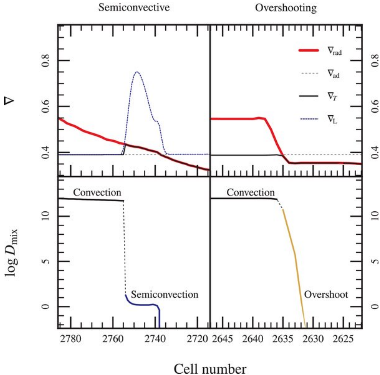
Figure 11. from Modules for Experiments in Stellar Astrophysics (MESA): Planets, Oscillations, Rotation, and Massive Stars Paxton et al. 2013 ApJS 208 4 doi:10.1088/0067-0049/208/1/4 https://dx.doi.org/10.1088/0067-0049/208/1/4 © 2013. The American Astronomical Society. All rights reserved.
