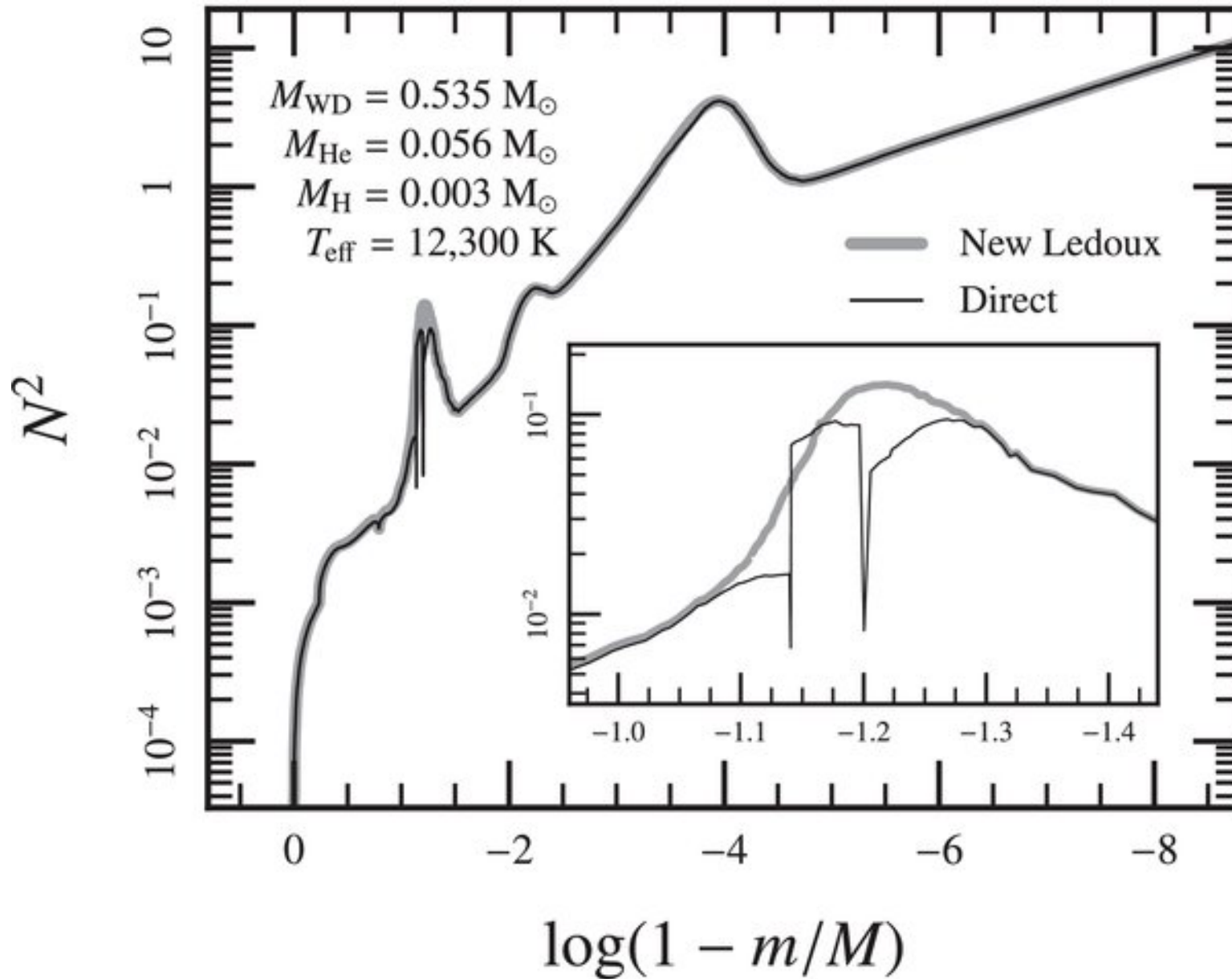
Figure 10. from Modules for Experiments in Stellar Astrophysics (MESA): Planets, Oscillations, Rotation, and Massive Stars Paxton et al. 2013 ApJS 208 4 doi:10.1088/0067-0049/208/1/4 https://dx.doi.org/10.1088/0067-0049/208/1/4 © 2013. The American Astronomical Society. All rights reserved.
