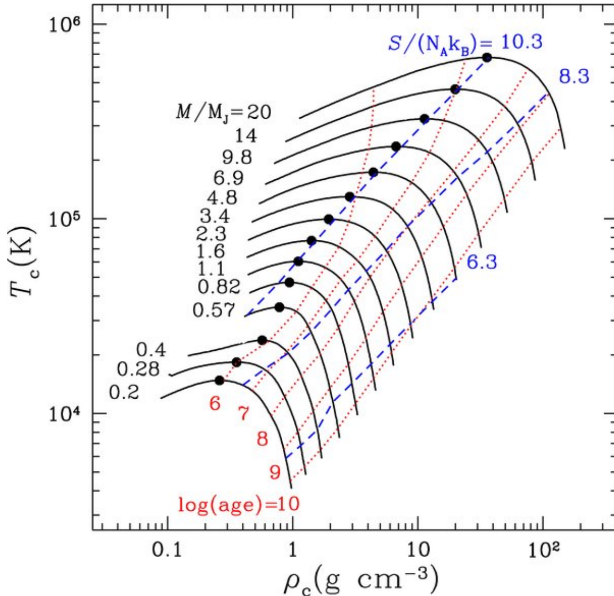
Figure 1. from Modules for Experiments in Stellar Astrophysics (MESA): Planets, Oscillations, Rotation, and Massive Stars Paxton et al. 2013 ApJS 208 4 doi:10.1088/0067-0049/208/1/4 https://dx.doi.org/10.1088/0067-0049/208/1/4 © 2013. The American Astronomical Society. All rights reserved.
