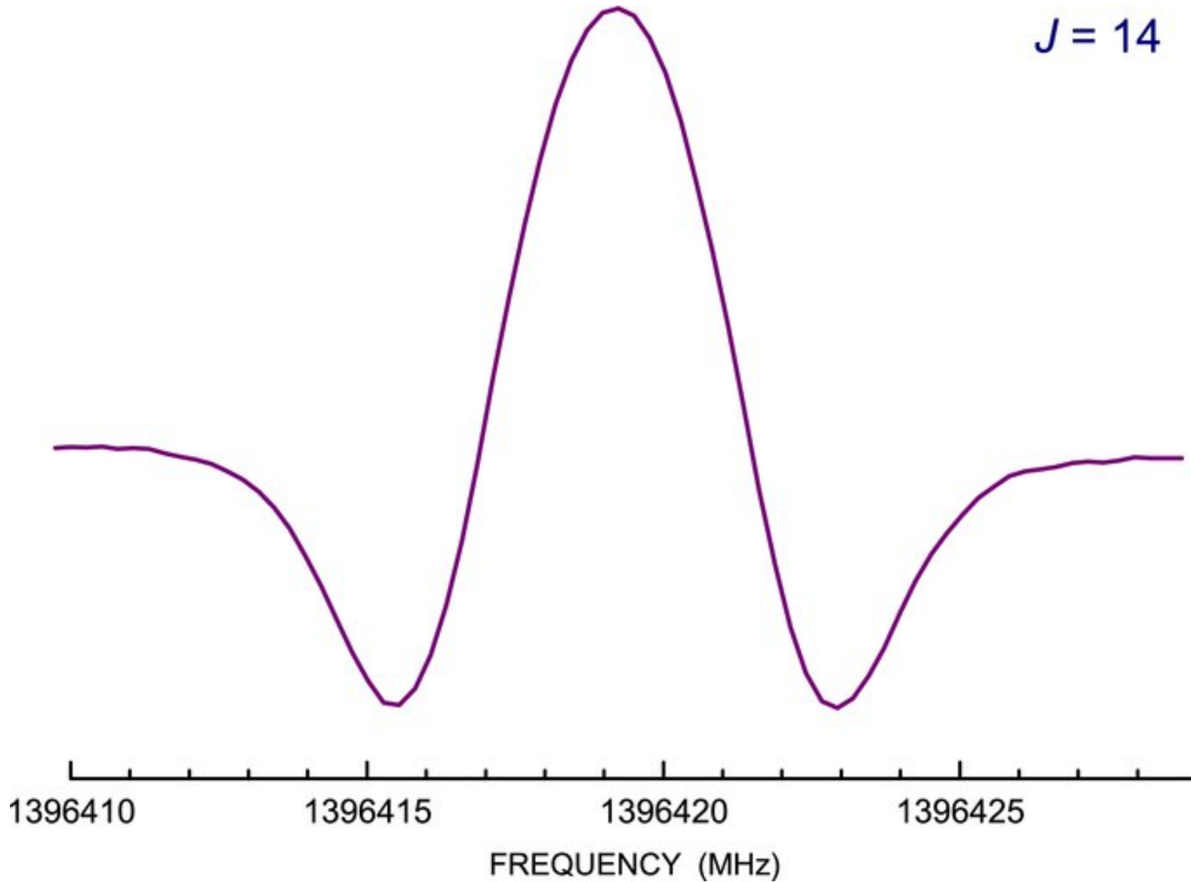
Figure 2. from Precise THz Measurements of HCO + , N 2 H + , and CF + for Astrophysical Observations Cazzoli et al. 2012 ApJS 203 11 doi:10.1088/0067-0049/203/1/11 https://dx.doi.org/10.1088/0067-0049/203/1/11 © 2012. The American Astronomical Society. All rights reserved.
