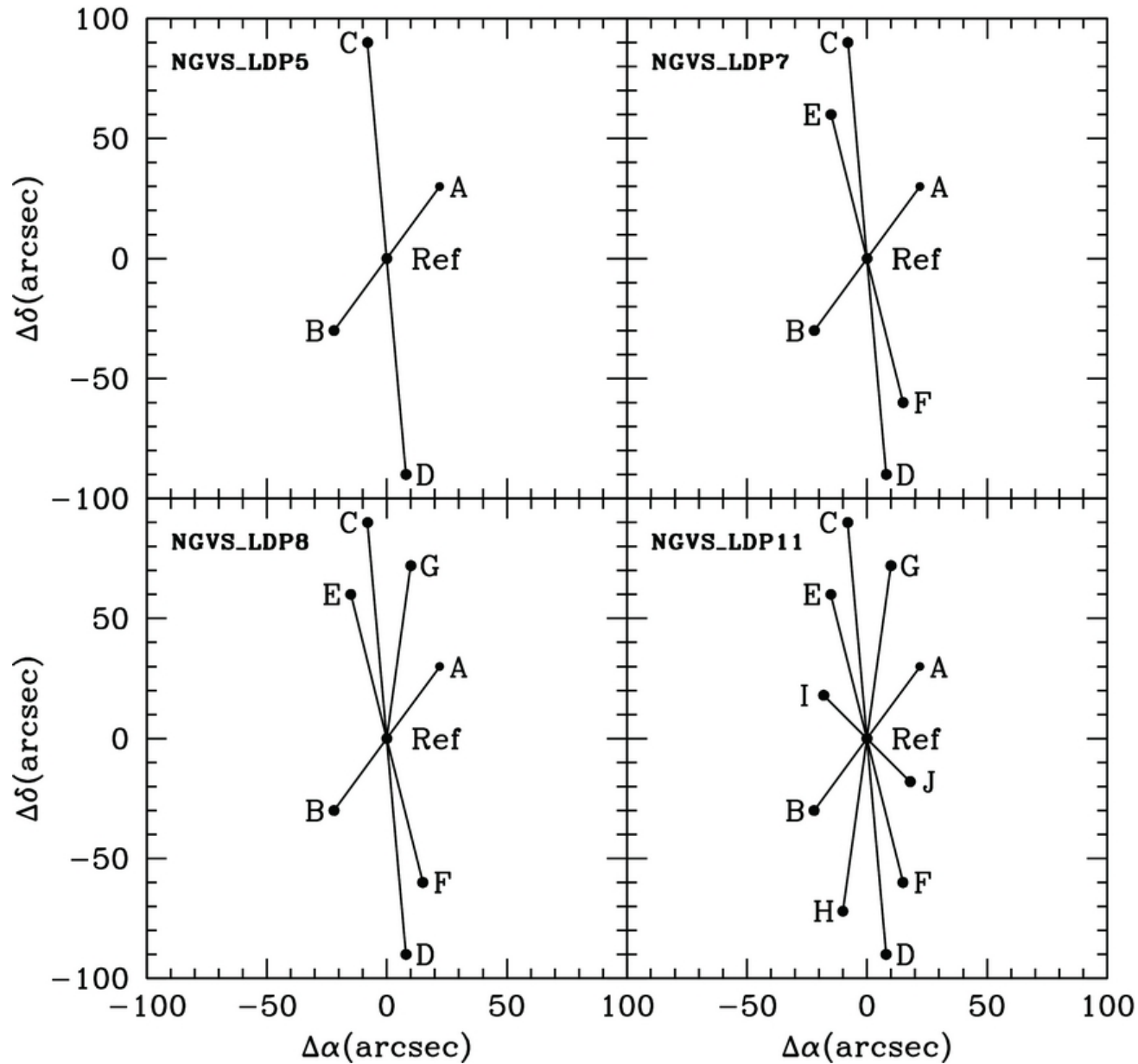
Figure 9. from The Next Generation Virgo Cluster Survey (NGVS). I. Introduction to the Survey Ferrarese et al. 2012 ApJS 200 4 doi:10.1088/0067-0049/200/1/4 https://dx.doi.org/10.1088/0067-0049/200/1/4 © 2012. The American Astronomical Society. All rights reserved.
