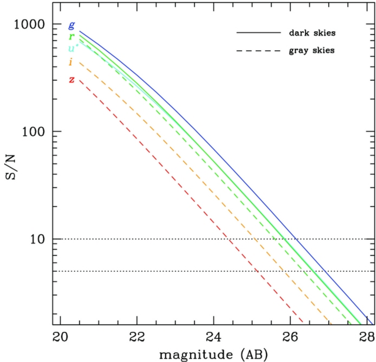
Figure 7. from The Next Generation Virgo Cluster Survey (NGVS). I. Introduction to the Survey Ferrarese et al. 2012 ApJS 200 4 doi:10.1088/0067-0049/200/1/4 https://dx.doi.org/10.1088/0067-0049/200/1/4 © 2012. The American Astronomical Society. All rights reserved.
