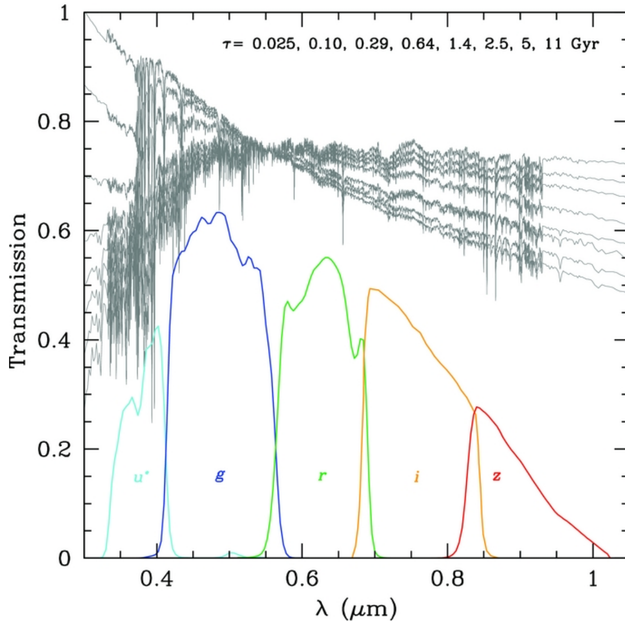
Figure 6. from The Next Generation Virgo Cluster Survey (NGVS). I. Introduction to the Survey Ferrarese et al. 2012 ApJS 200 4 doi:10.1088/0067-0049/200/1/4 https://dx.doi.org/10.1088/0067-0049/200/1/4 © 2012. The American Astronomical Society. All rights reserved.
