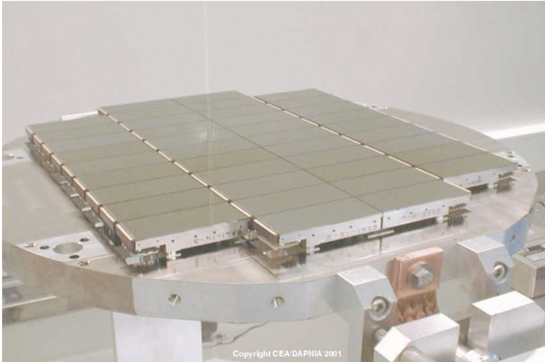
Figure 3. from The Next Generation Virgo Cluster Survey (NGVS). I. Introduction to the Survey Ferrarese et al. 2012 ApJS 200 4 doi:10.1088/0067-0049/200/1/4 https://dx.doi.org/10.1088/0067-0049/200/1/4 © 2012. The American Astronomical Society. All rights reserved.
