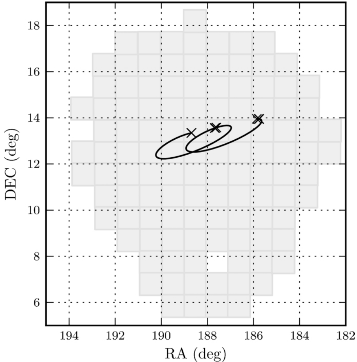
Figure 25. from The Next Generation Virgo Cluster Survey (NGVS). I. Introduction to the Survey Ferrarese et al. 2012 ApJS 200 4 doi:10.1088/0067-0049/200/1/4 https://dx.doi.org/10.1088/0067-0049/200/1/4 © 2012. The American Astronomical Society. All rights reserved.
