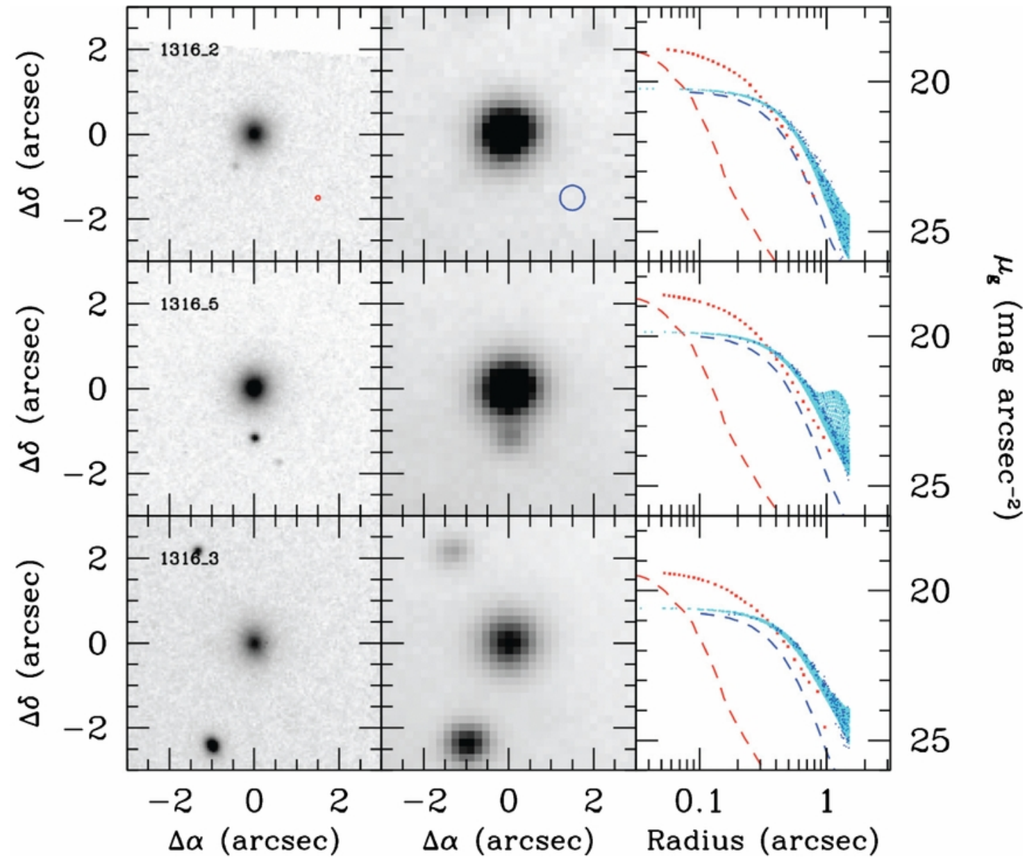
Figure 20. from The Next Generation Virgo Cluster Survey (NGVS). I. Introduction to the Survey Ferrarese et al. 2012 ApJS 200 4 doi:10.1088/0067-0049/200/1/4 https://dx.doi.org/10.1088/0067-0049/200/1/4 © 2012. The American Astronomical Society. All rights reserved.
